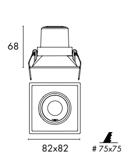
511D + HLP06
