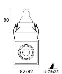
511D + 1LHG-300
