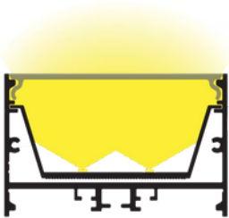
270011007 Reflector aluminio Aluminium reflector 75° -15% lm
