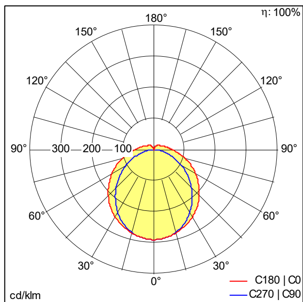
D44080AA_TECTON_B_BASIC_LED5200-840_L1522_LDE_WH.Idt
